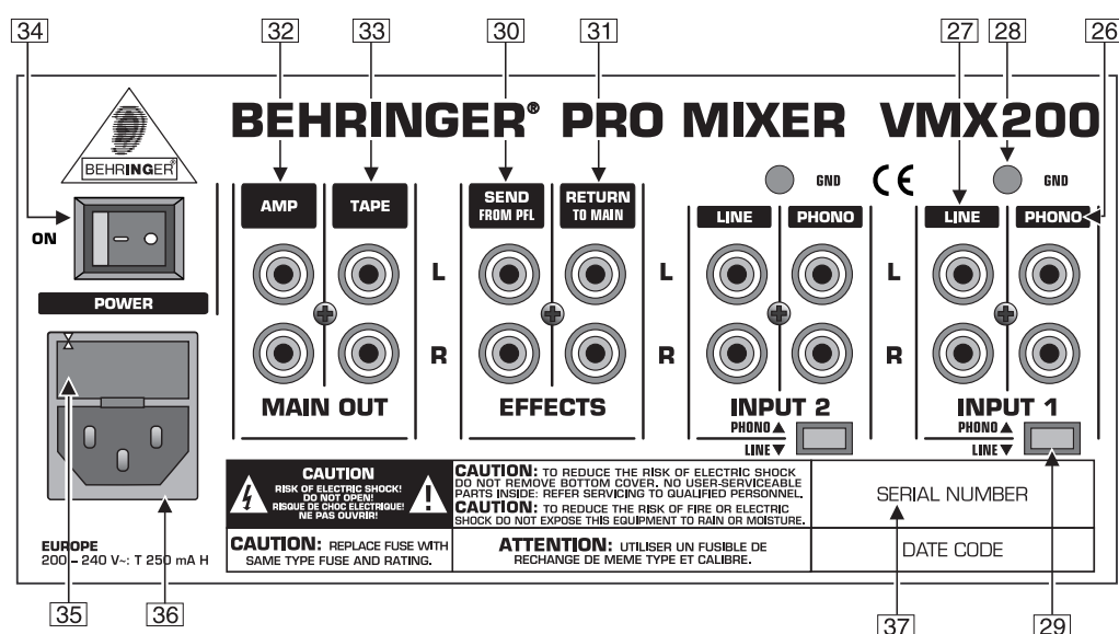
Fig 3.1: Rear view of the PRO MIXER VMX200
